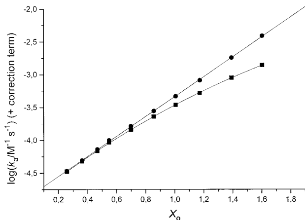
Figure 1. Excess acidity plots [Eqns (1) and (2)] for the \text{Ad}_{\text{E}2} hydration of 3-nortricyclanol ( 2-OH ) in \text{HClO}_4(\text{aq.}) at 318.2 K: (■) Eqn. (1); (●) Eqn. (2). The correction term, -\log[c_S/(c_S + c_{\text{S}^+\text{H}})] , was calculated with Eqn. (4) from the m' and \text{p}K_{\text{S}^+\text{H}} values in Table 2
